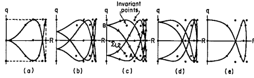
FIG. 1. Packet traces in the R - q plane. (Case \Delta n=3, \Delta n=2 .)
