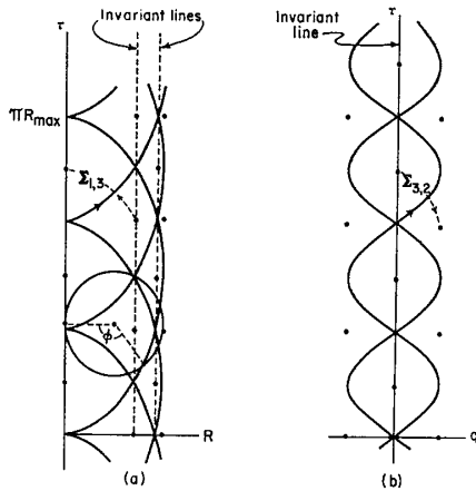
FIG. 2. Packet traces in the (a) R-\tau and (b) \tau-q planes. (Case \Delta n=3 , \Delta n=2 .)
