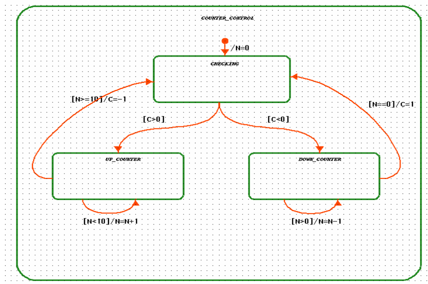
Figure 2: Statechart showing up-down counter
